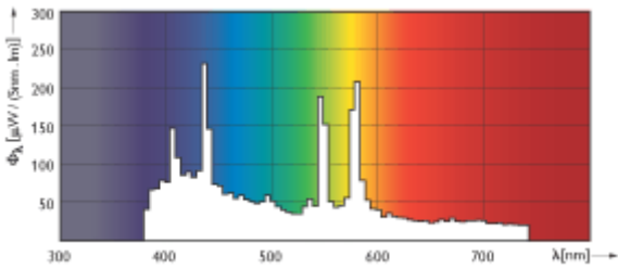
MSR Gold 400W SA/2 DE
